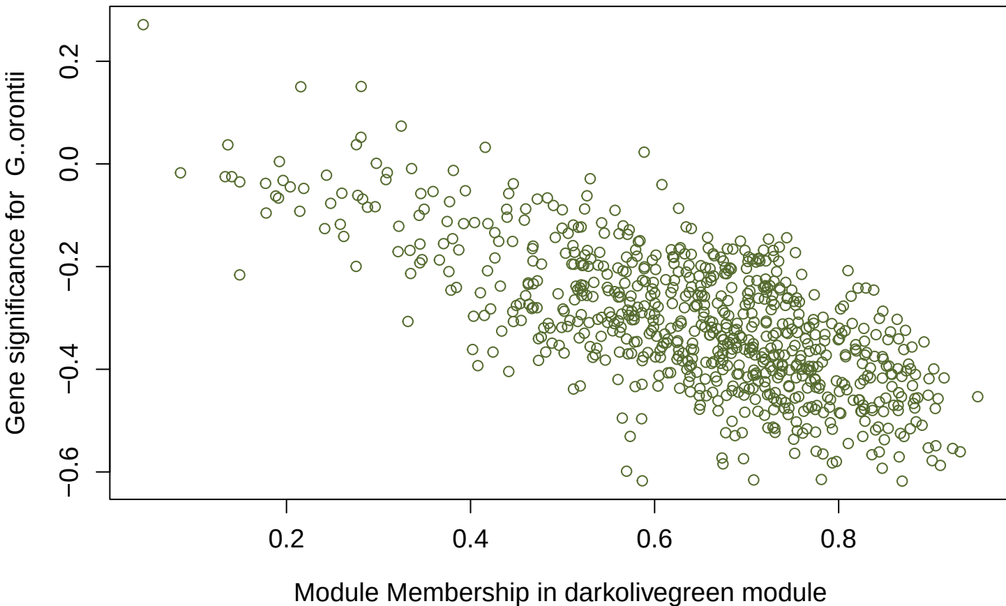
Module membership vs. gene significance cor=-0.69, p=2.7e-104
